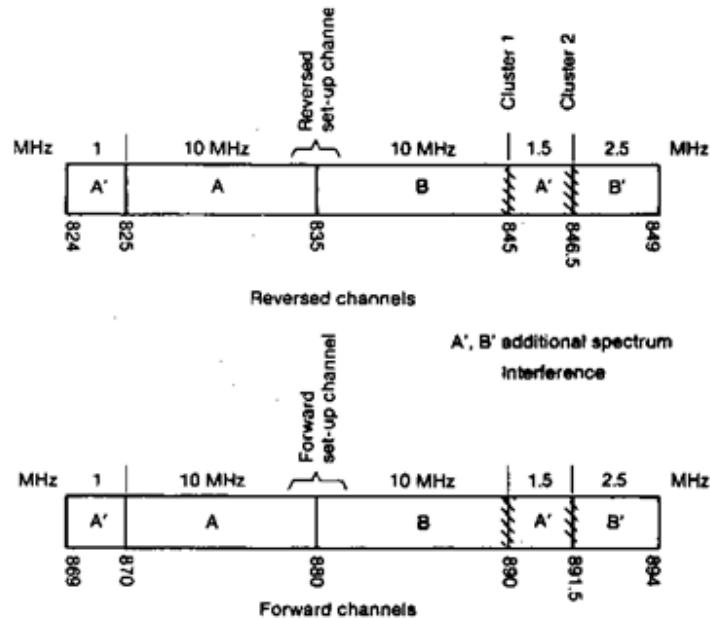
Fig. 12.1 Spectrum allocation with new additional spectrum.
