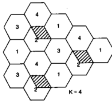
Fig. 4.4 Interference with frequency reuse pattern K=4 .
