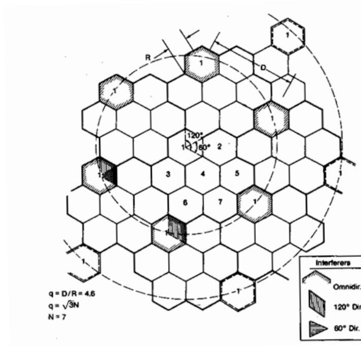
Fig.4.2. Interfering cells shown in a seven cell system (two-tiers)
