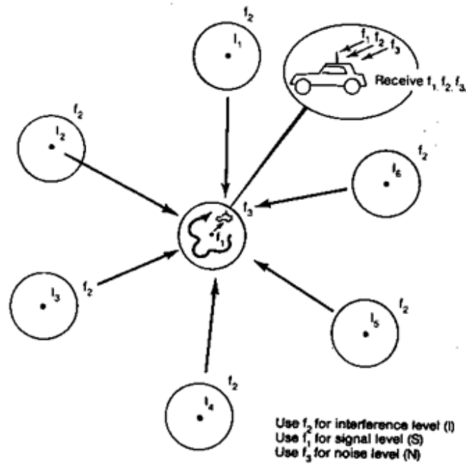
Fig.1 Test -1 cochannel interference at mobile unit.
