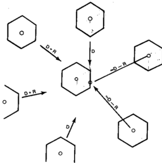
Fig.3. Cochannel interference (a worst case)
